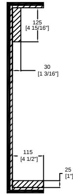
B-B VIEW
