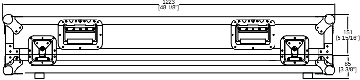
BACK VIEW
