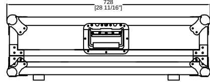
RIGHT VIEW
