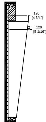
D-D VIEW
