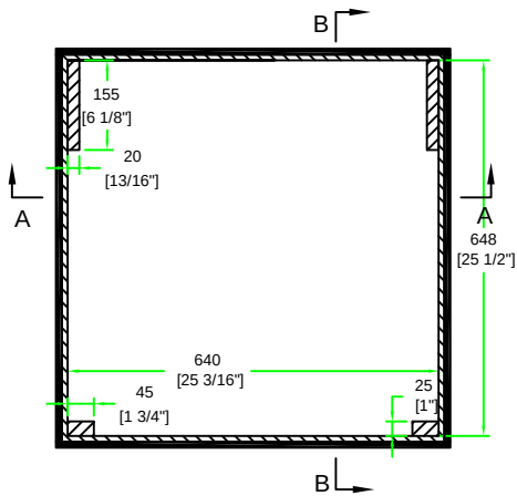
B-B VIEW
