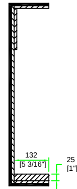
B-B VIEW
