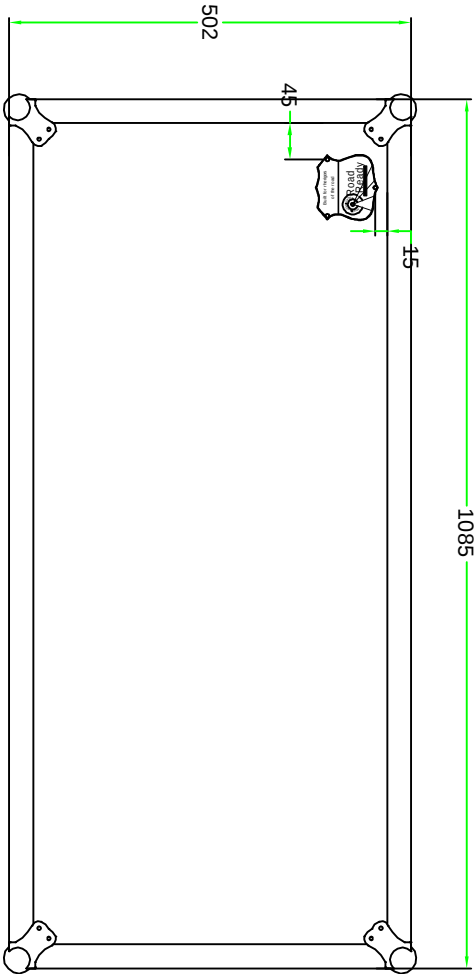
TOP VIEW
