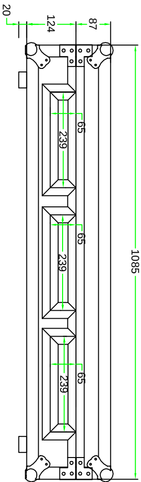
FRONT VIEW
