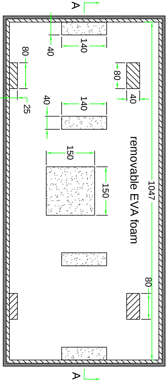
TOP VIEW OF COVER
