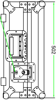
LEFT VIEW
