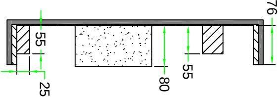
B-B VIEW
