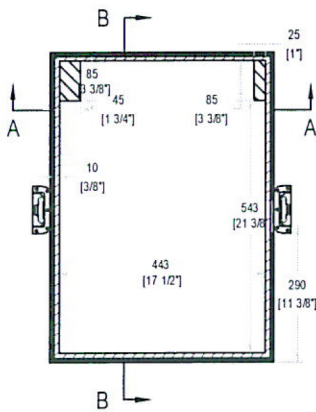
TOP VIEW OF BASE
