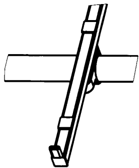
detail A 1:5
