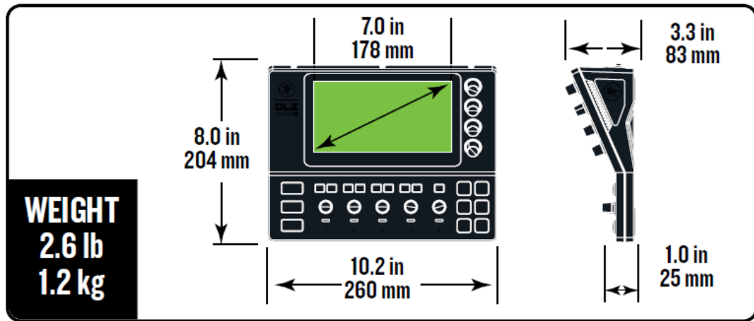
DLZ Creator XS Dimensions
