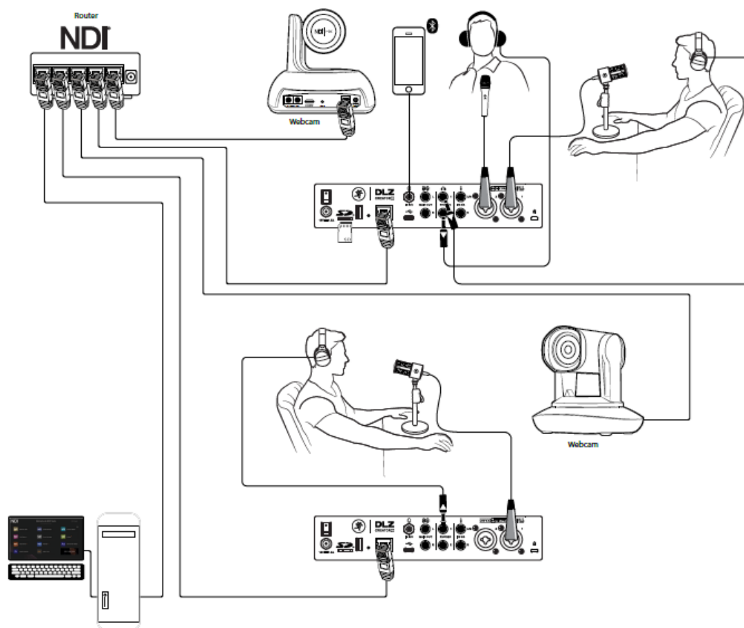
接続図 2 – DLZ Creator XS から DLZ Creator XS
