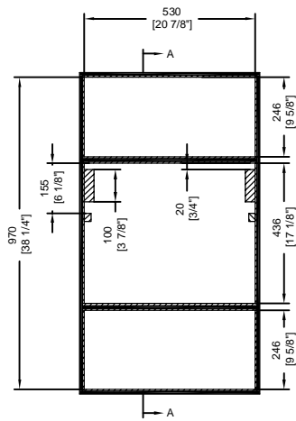
Top view of Base
