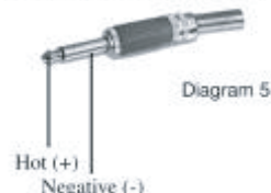
Unbalanced TS 1/4" Plug
