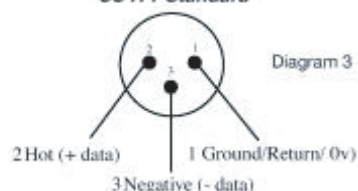
Male XLR Pin Configuration: US ITT Standard
