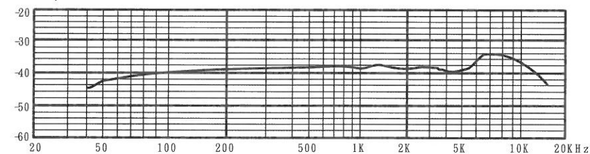
Frequency Response Graph
