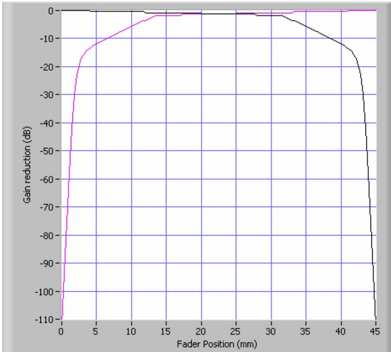
Cross-fader curves - logarithmic gain reduction
